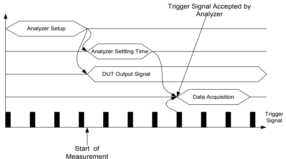
Fig. 4-42 Test with stationary test signal and periodic trigger signal
