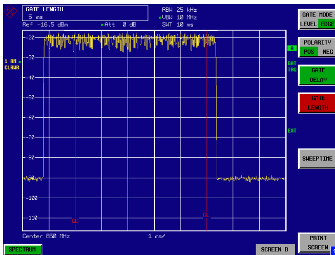
Fig. 2-30 Setting the parameters Gate Delay and Gate Length in time domain. The time interval required to measure the spectrum is indicated by two vertical lines.
