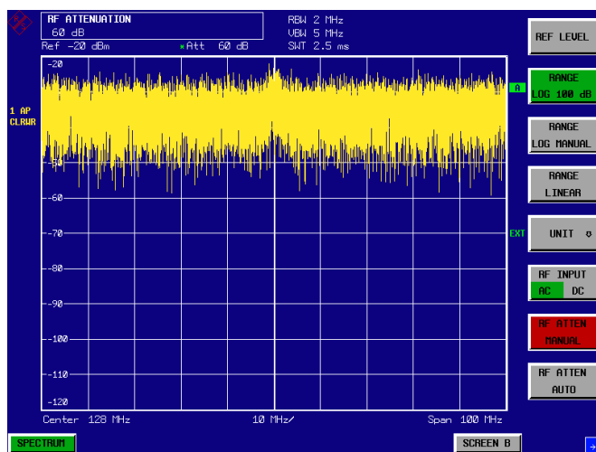
Fig. 2-9 Sinewave signal with low S/N ratio. The signal is measured with the autopeak detector and is completely swamped by the intrinsic noise of the Spectrum Analyzer.
