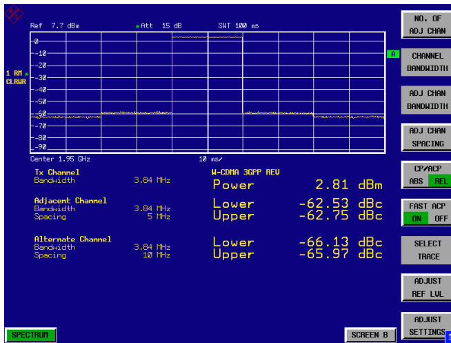
Fig. 2-33 Measuring the adjacent channel power of a W-CDMA signal with the Fast ACP method
